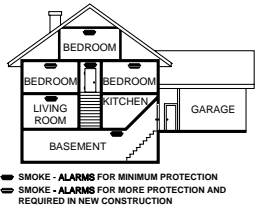
Figure 3: Recommended smoke-alarm protection for a multi-level residence:
