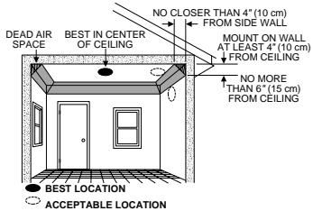
Figure 4: Recommended smoke-alarm mounting locations:
